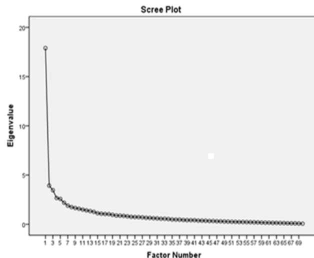
Fig 1: Scree Plot
