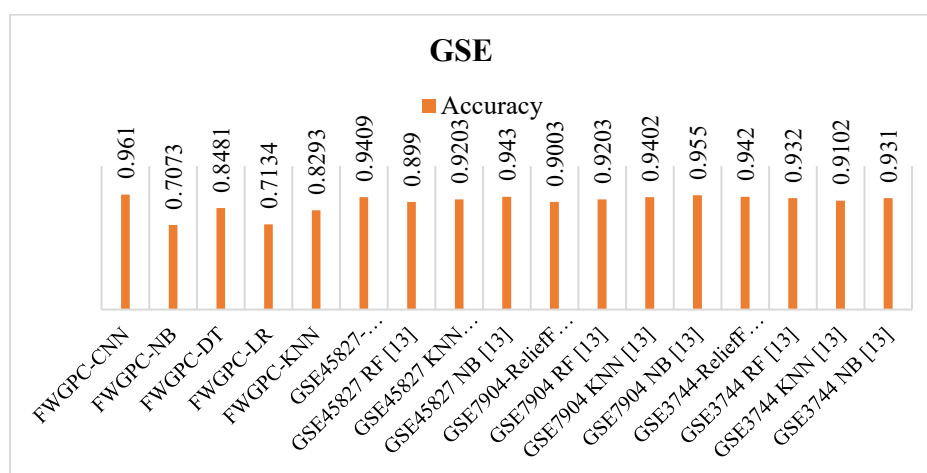
Figure 11: Comparison of the proposed method with previous methods in terms of accuracy criteria on the GSE dataset.
