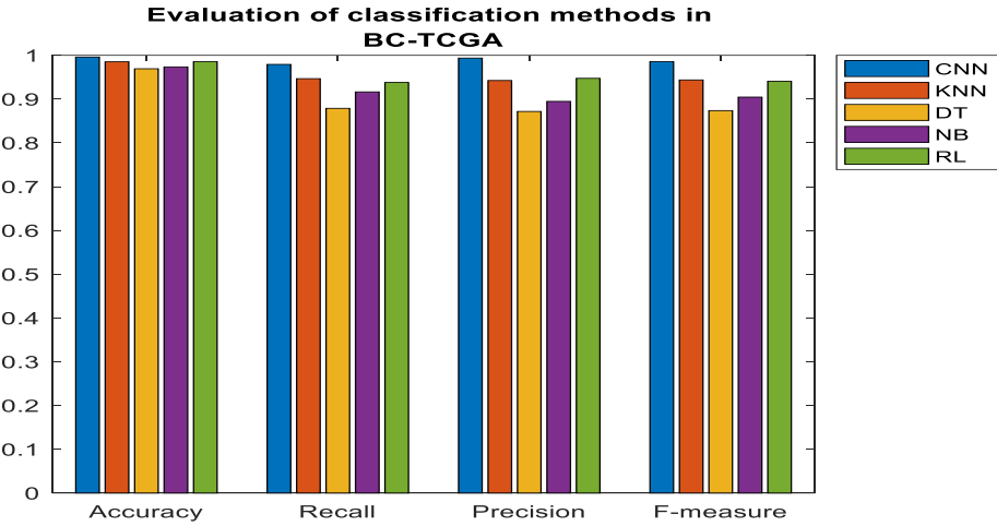
Figure 4: Bar chart comparing the average evaluation criteria for classification methods on the dataset (a) BC-TCA (b) GSE
