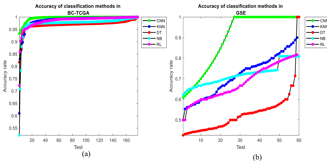
Figure 5: Comparison of the accuracy of the proposed method with classification algorithms on the datasets (a) BC-TCGA (b) GSE
